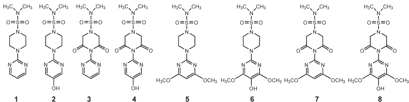
Figure 2. Analogues of N,N' -dimethyl-4-(pyrimidin-2-yl)piperazine-1-sulfonamide ( 1 ) synthesized and evaluated.
