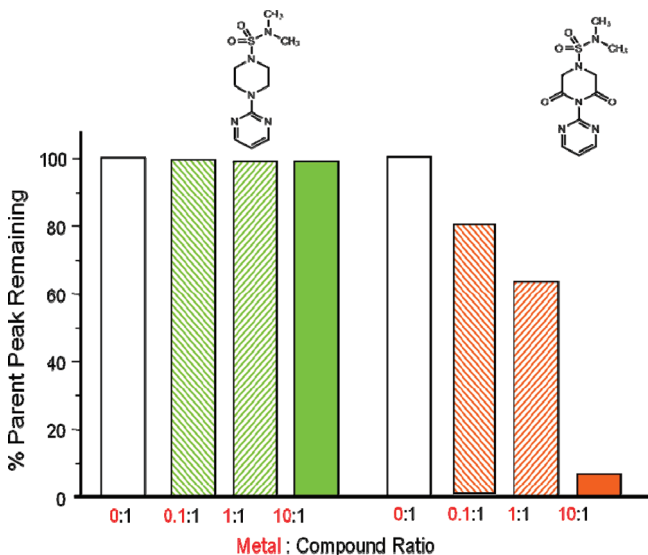
Figure 3. ESI-MS analysis of parent peak of N,N' -dimethyl-4-(pyrimidin-2-yl)piperazine-1-sulfonamide ( 1 ) and N,N' -dimethyl-3,5-dioxo-4-(pyrimidin-2-yl)piperazine-1-sulfonamide ( 3 ) in the presence of increasing amounts of Fe 2+ solutions.
