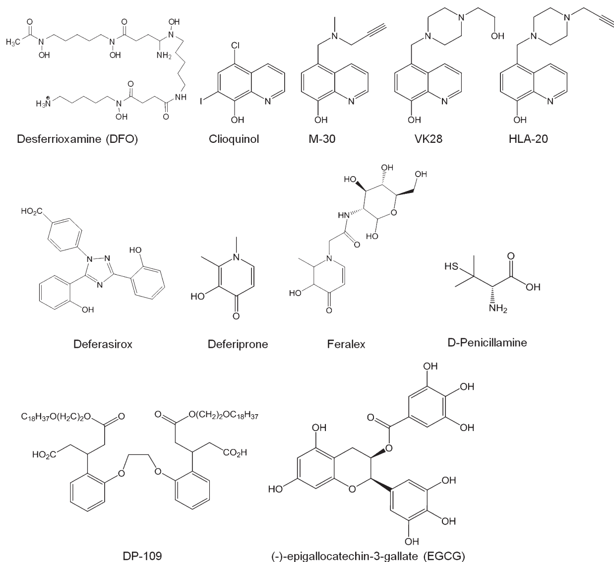
Figure 1. Structure of antioxidant and chelators evaluated for cataract, AMD, and AD.
